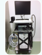
Raman
